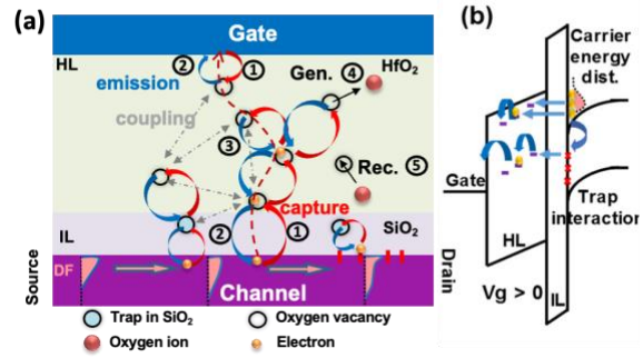
Fig. 1(a) Trap behaviors: (1) charge trapping (2) charge detrapping (3) trap coupling (4) trap generation and (5) recombination induced degradation in the gate dielectrics simulated by 3D-KMC method. (b) the energy band diagram of charge trapping in the nMOSFET with the interfacial layer (IL) and high k layer (HL) under stress considering the impact of carrier energy distribution.
