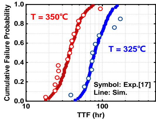
Fig.12 Calibration of cumulative failure distribution between simulation and experimental data [17] at different temperatures.
