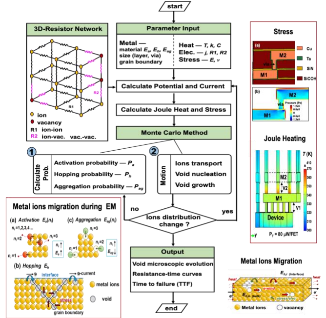
Fig. 11 EM simulation flowchart by using 3D KMC method to simulate metal ions migration including the metal ions activation, hopping and aggregation.
