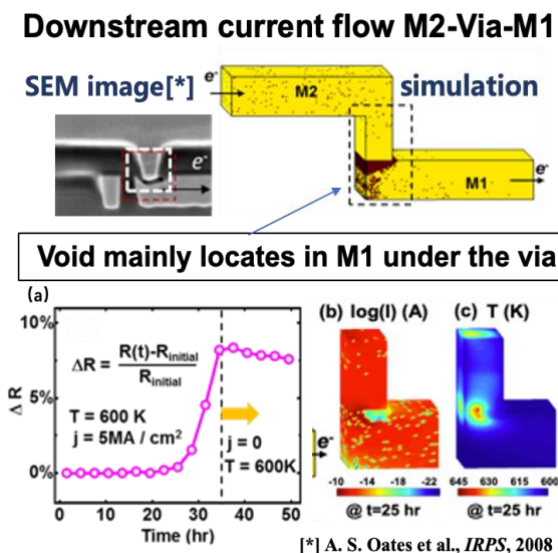
Fig.14 Downstream current flow from M2 to M1 in EM simulation. A void formed in M1 (compared with SEM image). (a) R-t curve (b)-(c) local current and temperature distribution of via-M1.
