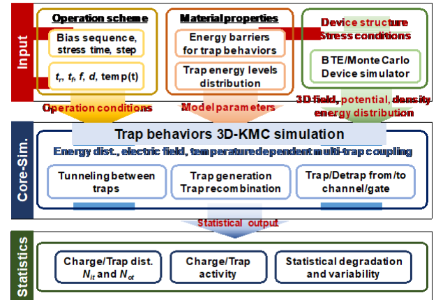
Fig.2 3D-KMC based reliability simulation framework[4,7,8]
