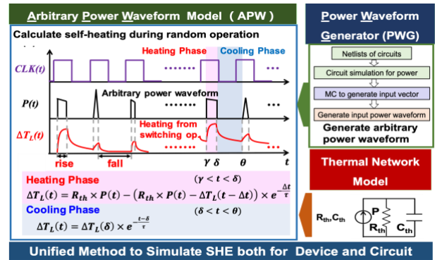
Fig.3 Framework of the unified method to simulate SHE both for device and circuit. Arbitrary power waveform (APW) self-heating model to calculate self-heating at the arbitrary operation conditions.[4,7,8]
