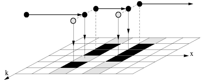
Fig. 1. The particle annihilation strategy attempts to minimize the weights stored in the mesh elements. The weights of the initial and continuing particle have the same sign to ensure current continuity. Particles and mesh elements carrying a positive weight are in black, the ones carrying a negative weight are in grey.
