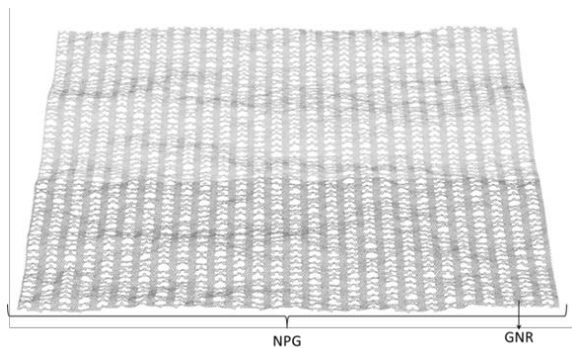
Fig. 1. NPGs are made as 2D arrays of laterally connected parallel GNRs.
