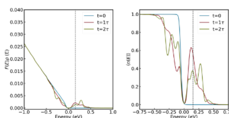
Fig. 2. Time and energy resolved phonon absorption in monolayer graphene.
