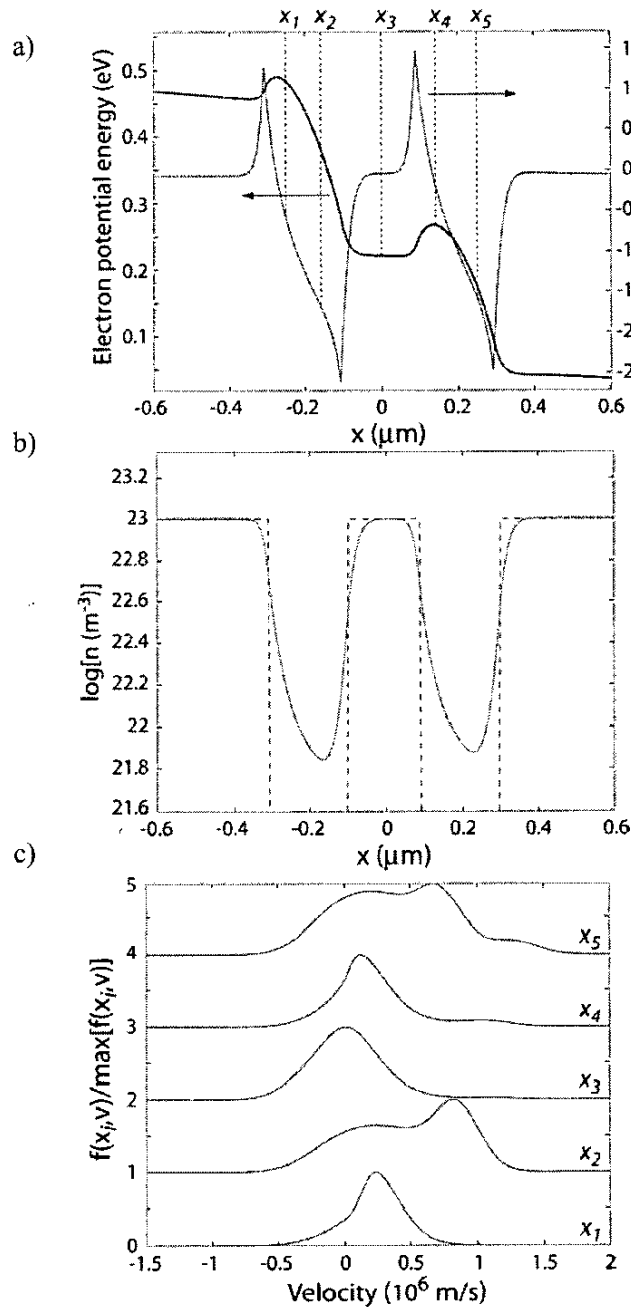
Fig. 1: (a) Electron potential energy and electric field. The labels x_i mark the points in space for which the electron distribution functions in Fig. 1(c) are plotted. (b) Electron density (solid line) and doping density (dashed line, whole range not shown). (c) Normalized electron distribution function. The parameters in the calculation are: The doping densities N^+ = 10^{23} \text{ m}^{-3} , N^- = 10^{19} \text{ m}^{-3} , the effective mass m^* = 0.067m_0 , the scattering time \tau = 2.5 \cdot 10^{-13} \text{ s} . The central N^-N^+N^- region has the dimensions 200/200/200 nm, the contact N^+ regions are 1 \mu\text{m} long.
