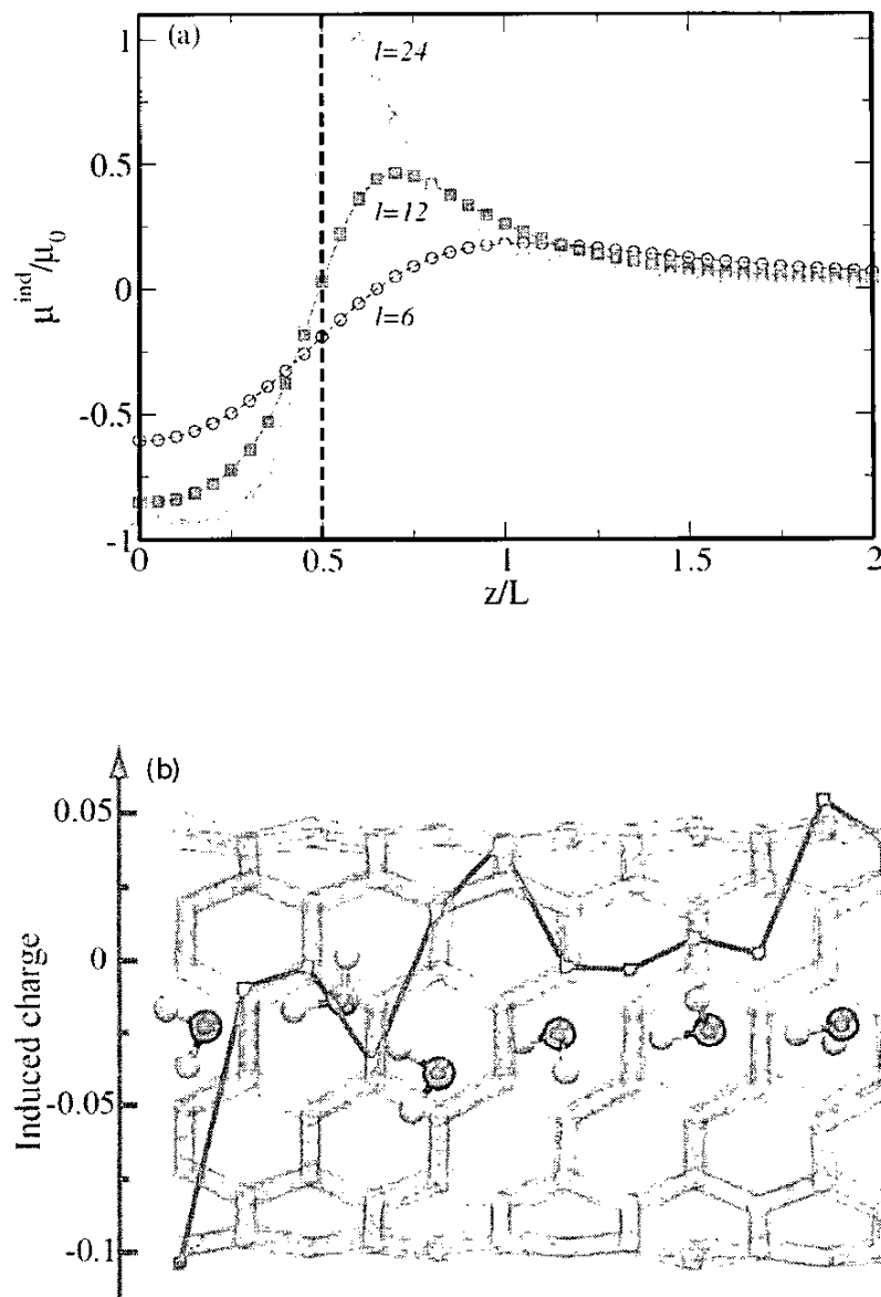
Figure 1: (a) The ratio of the induced dipole \mu^{ind} to an external dipole \mu_0 positioned along the axis of a (6, 6) SWNT. The location of \mu_0 relative to the nanotube center z is scaled by the nanotube length L with 6, 12, 24 sections respectively. The dashed line indicates the right end of the finite SWNT. (b) The background is a snapshot taken from a MD simulation of a 6-water-wire inside a (6, 6) nanotube segment with 12 sections. The overlaying curve plots the summed induced surface charges (in squares) of each section of the nanotube.
