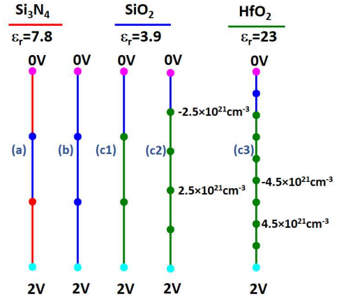
Figure 1: Gate stacks studied in this paper. Mesh points are showed in dots. Color legend of each material is shown on top with its relative dielectric constant. Fixed charge is also added to certain nodes.
