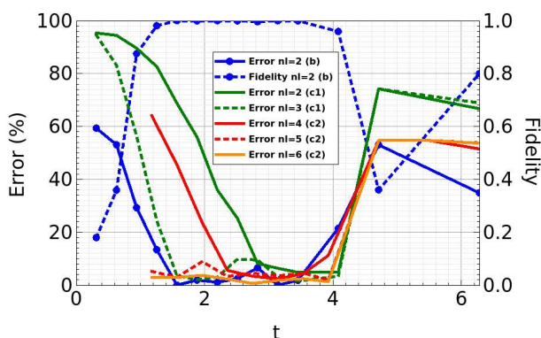
Figure 8: Simulated QC fidelity and error as a function of t and n_i of structures (b), (c1), and (c2). Error is defined by the average relative absolute error.
