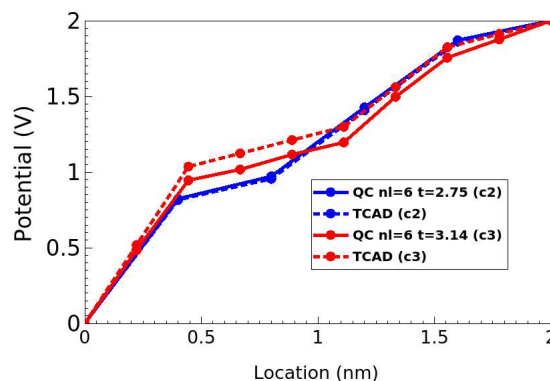
Figure 9: Best solutions obtained from QC simulation and TCAD for structures (c2) and (c3).
