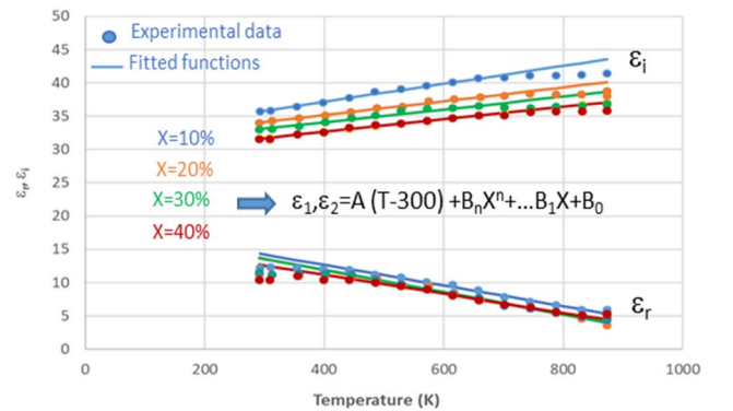
Fig. 4: Experimental permittivity variations (symbols) and fits (lines) versus temperature and Ge concentration. The polynomial function extracted from these results is given on the graph. All the constants A, B 0 , ... B n , are T and X-independent.
