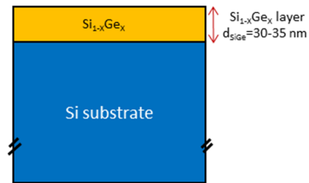
Fig. 1: Experimental stack used for \text{Si}_{1-x}\text{Ge}_x parameter calibration.
