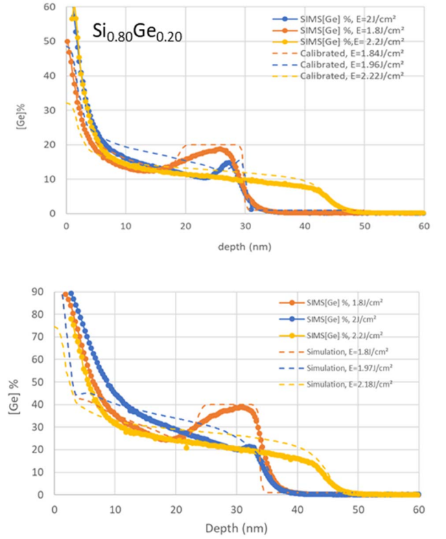
Fig. 6: Experimental and simulated concentration depth profiles in \text{Si}_{0.80}\text{Ge}_{0.20} and \text{Si}_{0.60}\text{Ge}_{0.40} samples annealed at laser energy density from 1.8 to 2.2 J/cm 2 .
