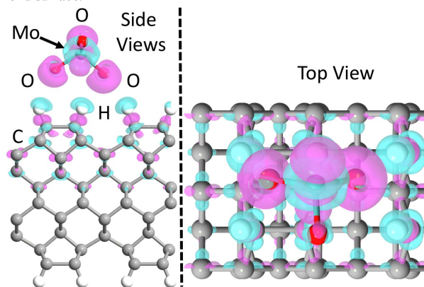
Figure 3. The (left hand side) side view and (right hand side) top view of charge density difference for the most stable \text{MoO}_3 -doped diamond surface. The purple regions represent electron accumulation and the green regions represent electron depletion (hole accumulation). The isosurface values are \pm 0.001 \text{ Bohr}^{-3} .
