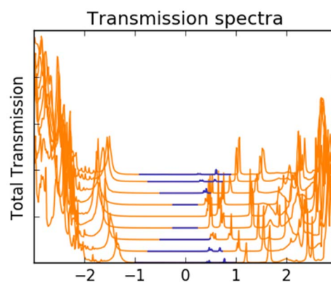
Figure 5. Series of transmission plots for Configuration A under different applied bias from -2.0V to 2.0V. From top to bottom, the blue line illustrates the applied bias window at -2.0V, -1.5V, -1.0V, -0.5V, 0V, +0.5V, +1.0V, +1.5V, +2.0V.
