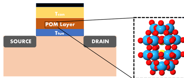
Figure 6. Conceptual device architecture for molecule-based charge trap flash memory cell. The POM cluster ( [W_{18}O_{54}(SO_3)_2]^{-4} ) is also illustrated where S=Yellow, W=Blue and O=Red.
