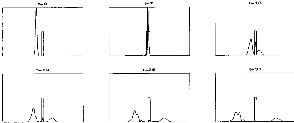
Figure 1: exact solution
